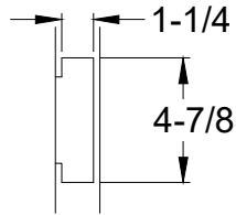
ASA Strike
