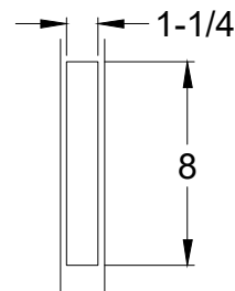
86 Mortise Lock
