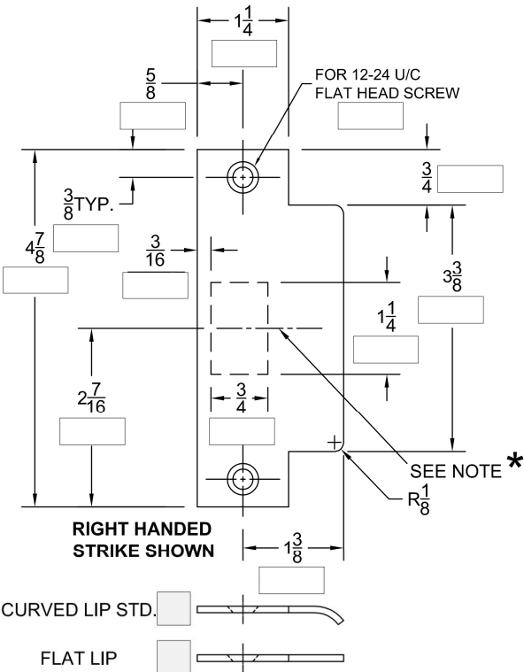
Custom "ASA" Strike
