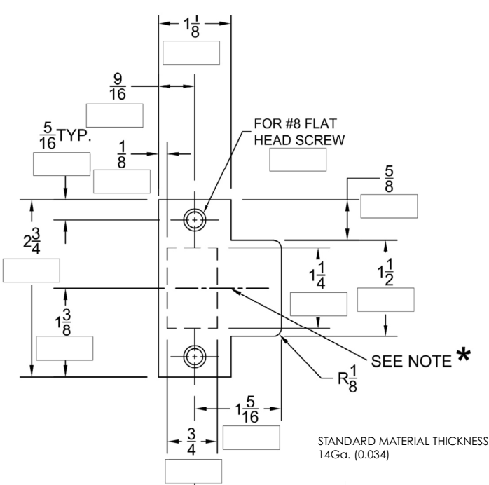
Custom "T" Strike
